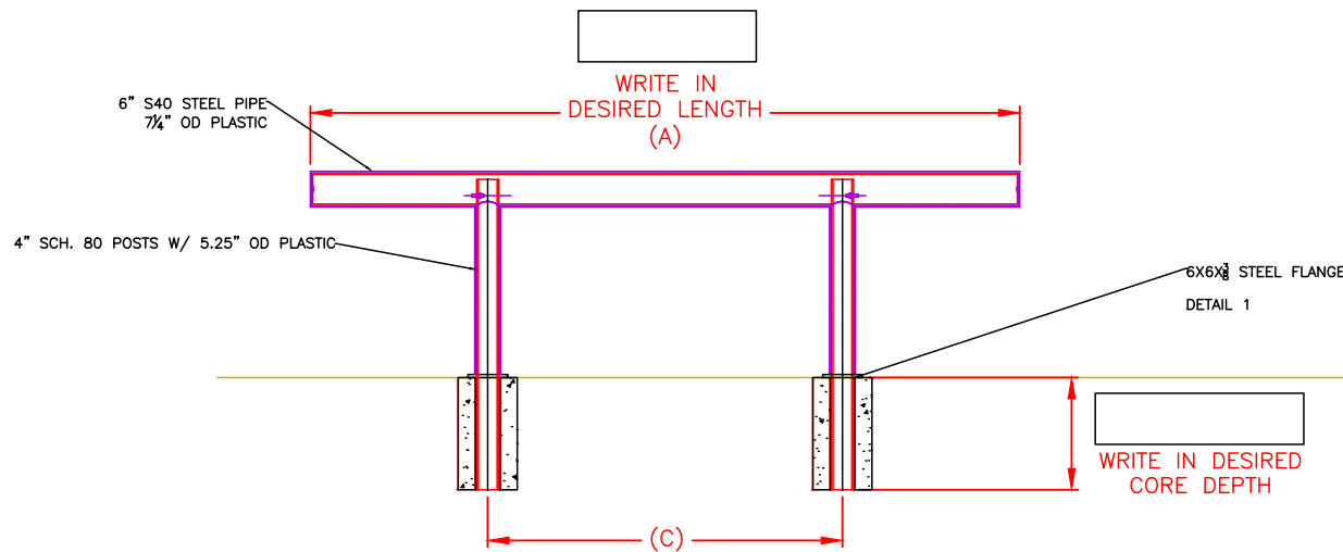
FRONT VIEW
