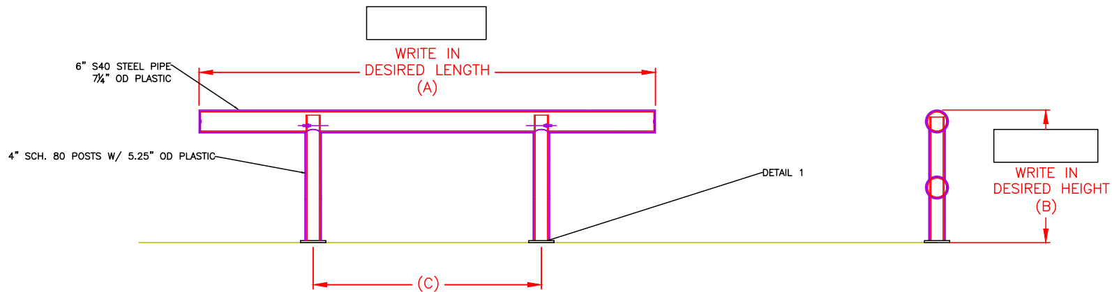
FRONT VIEW
