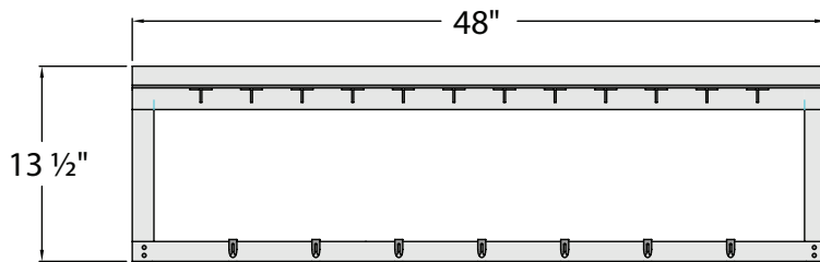
a. 1122PR | T-Bar Wall Shelf / Pot Rack
