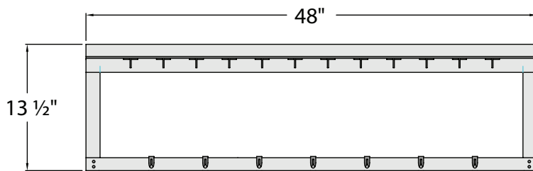
a. 1122PR | T-Bar Wall Shelf / Pot Rack
